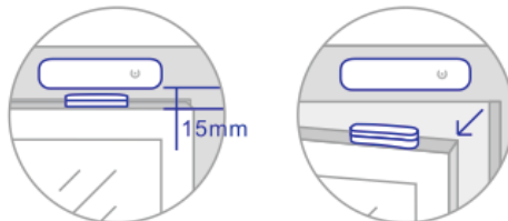
Horizontal Installation
